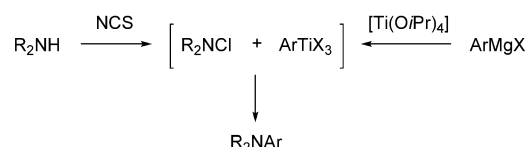
Scheme 1. Titanium-mediated amination of Grignard reagents. [Ti(OiPr) 4 ] with Grignard reagent provided the best yield of the desired product (Table 1, entry 6). [11]
